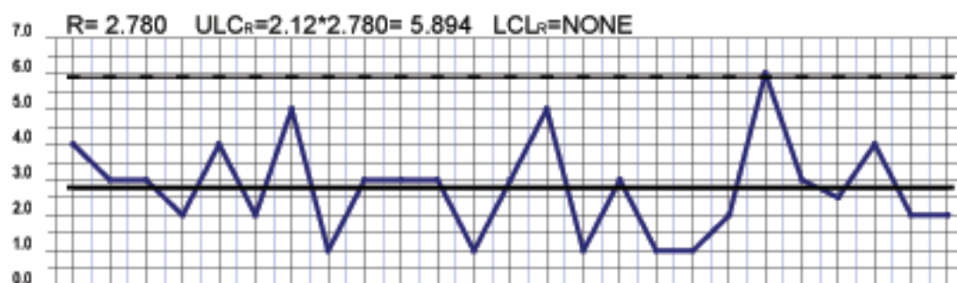
RANGES ( R CHART )
